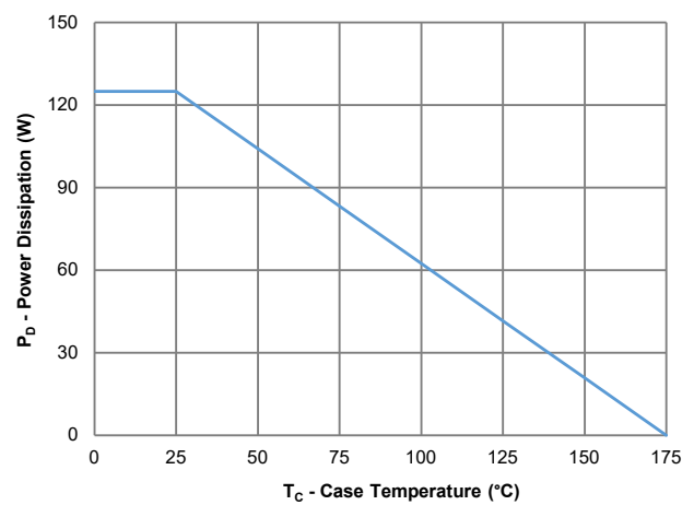
Figure 10: Power Derating
