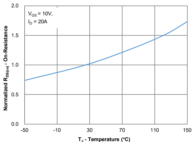
Rev. 1.2 Figure 5: On-Resistance vs. Junction Temperature
