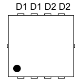
PIN Configuration (Top View)
