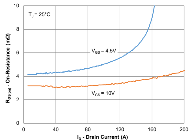
Figure 4: On-Resistance vs. Drain Current and Gate
