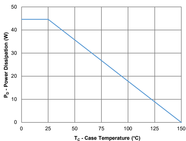
Figure 10: Power Derating
