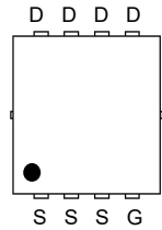
PIN Configuration (Top View)
