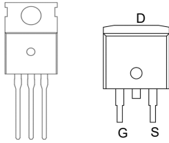
PIN Configuration
