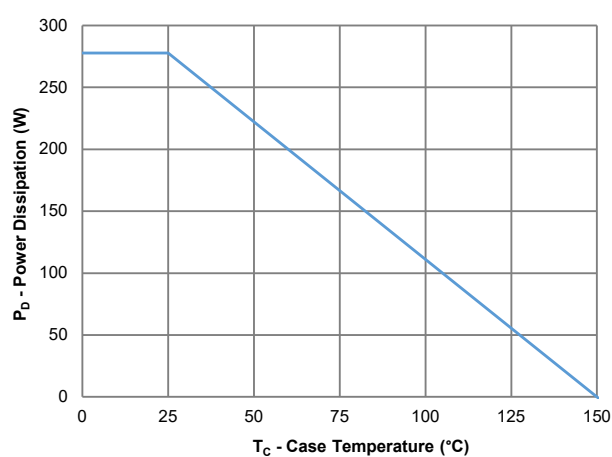
Figure 10: Power Derating
