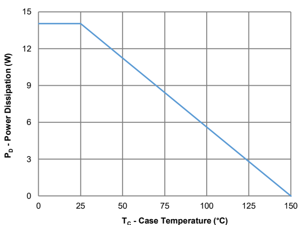
Figure 10: Power Derating
