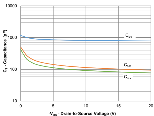
Figure 9: Capacitance Characteristics
