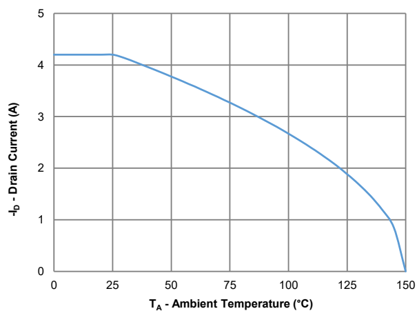
Figure 11: Current Derating
