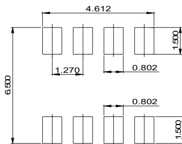
DIMENSIONS: MILLIMETERS
