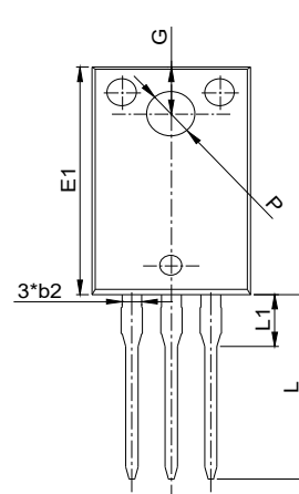
Bottom View
