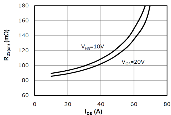
Fig 5: R_{DS(on)} vs. I_{DS} Characteristics ( T_J=25^{\circ}\text{C} )
