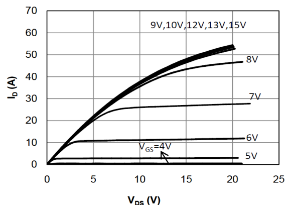
Fig 2. Output Characteristics ( T_J=150^{\circ}\text{C} )
