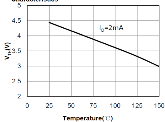
Fig 4: V_{TH} Vs. T_J Temperature Characteristics
