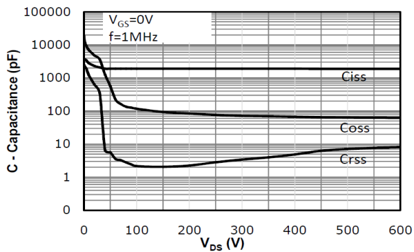
Fig 11: Capacitance Characteristics
