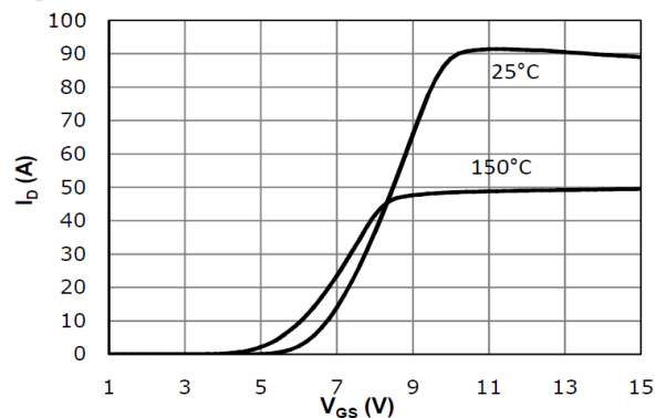
Fig 3: Transfer Characteristics
