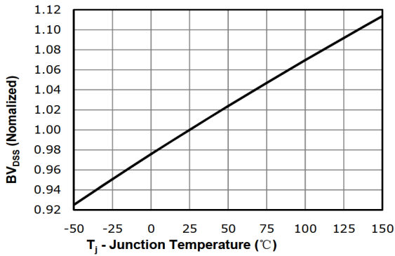
Fig 7: BV_{DSS} vs. Temperature
