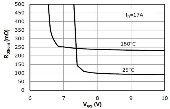
Fig 8: R_{DS(on)} vs. Gate Voltage
