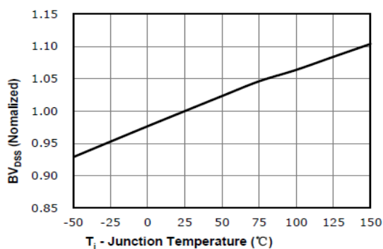
Fig 7: BV_{DS} vs. Temperature
