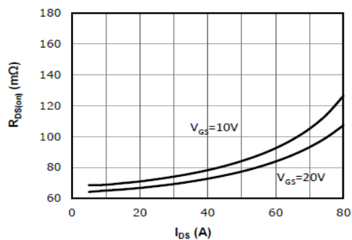
Fig 5: R_{DS(on)} vs. I_{DS} Characteristics ( T_j=25^\circ\text{C} )
