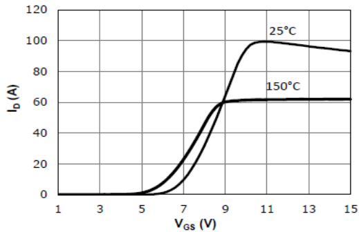
Fig 3: Transfer Characteristics
