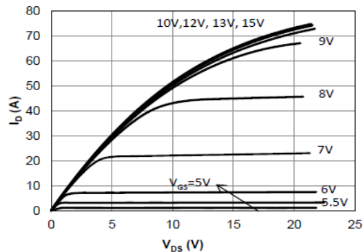
Fig 2: Output Characteristics ( T_j=150^\circ\text{C} )
