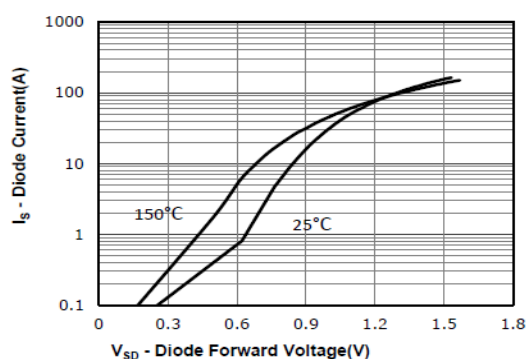
Fig 9: Body-diode Forward Characteristics
