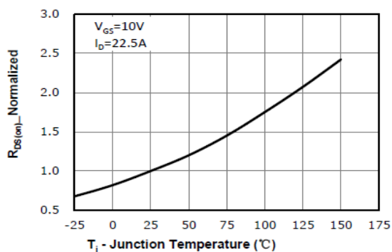
Fig 6: R_{DS(on)} vs. Temperature
