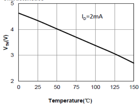
Fig 4: V_{TH} vs. T_j Temperature Characteristics
