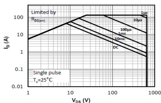
Fig 12: Safe Operating Area
