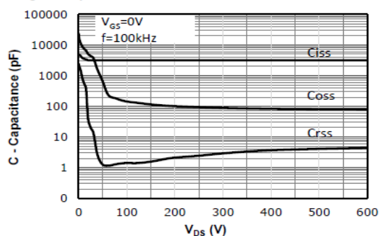
Fig 11: Capacitance Characteristics
