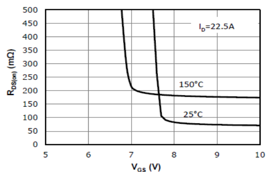
Fig 8: R_{DS(on)} vs. Gate Voltage
