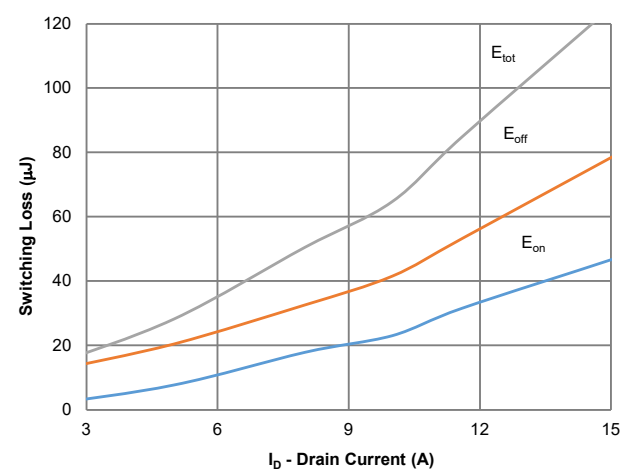
Figure 12: Switching Losses vs. Drain Current
