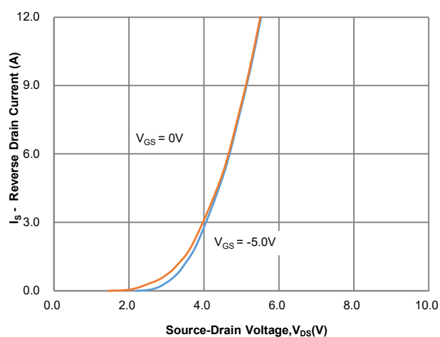
Figure 6: Body Diode Characteristic, T_J = 175^\circ\text{C}
